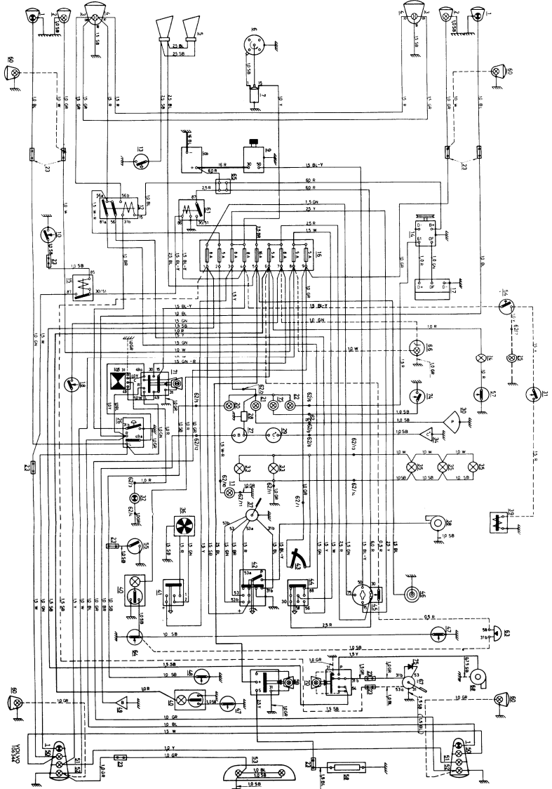
Illustration 3-C. Wiring diagram 145 carb. engine
