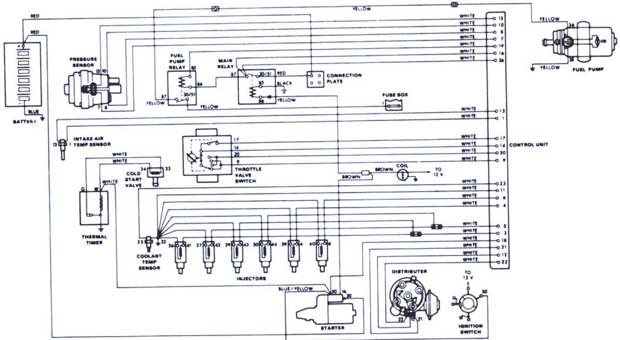
Wiring Diagram For Six Cylinder Cars
